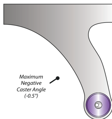
Figure 1 - Right Wheel configuration as viewed from front of car
